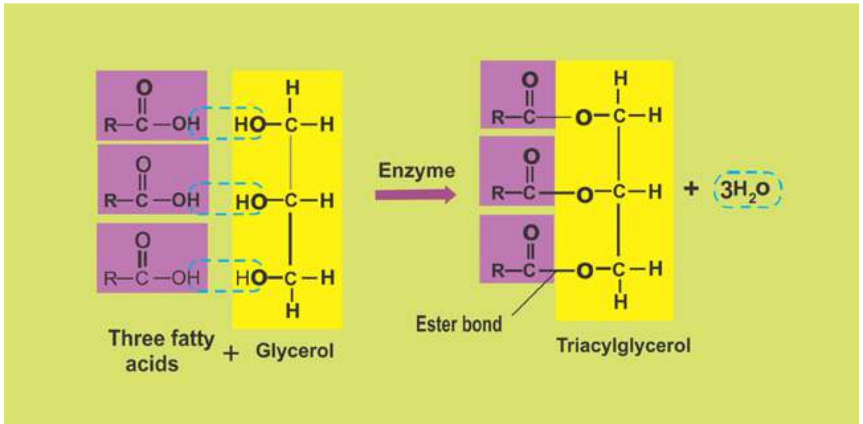
Fig. 2.7: Triacylglycerol is composed of one glycerol and three fatty acid molecules.
