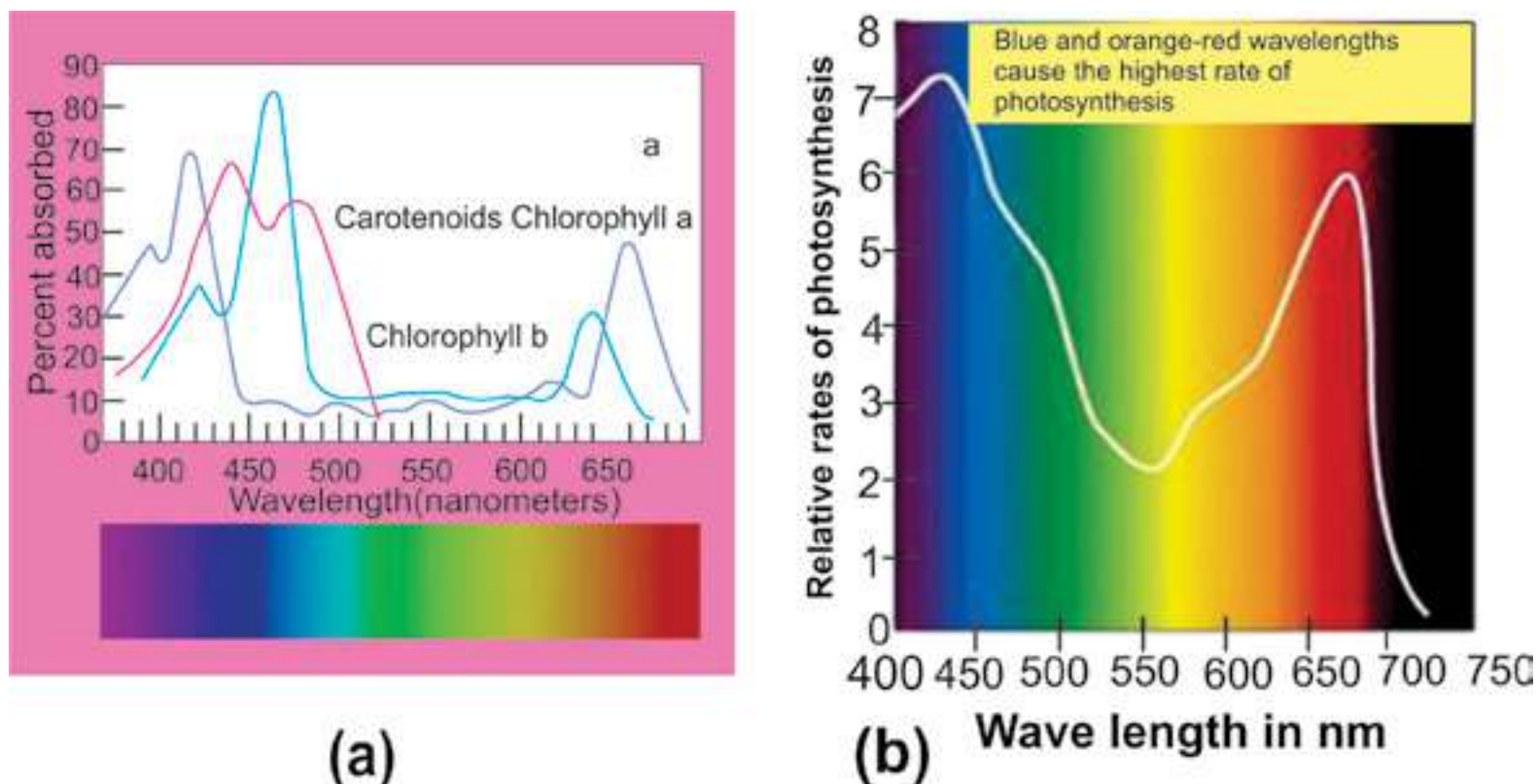
Fig. 11.4 (a) Absorption spectrum of chlorophyll and carotenoids. (b) Action spectrum for photosynthesis.
