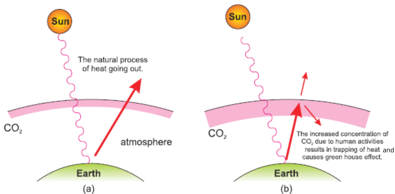
Fig.14.3: Greenhouse effect
