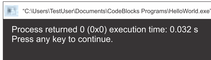
Figure 1.4: Program Output
