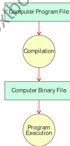
Figure 1.5: Program Execution
